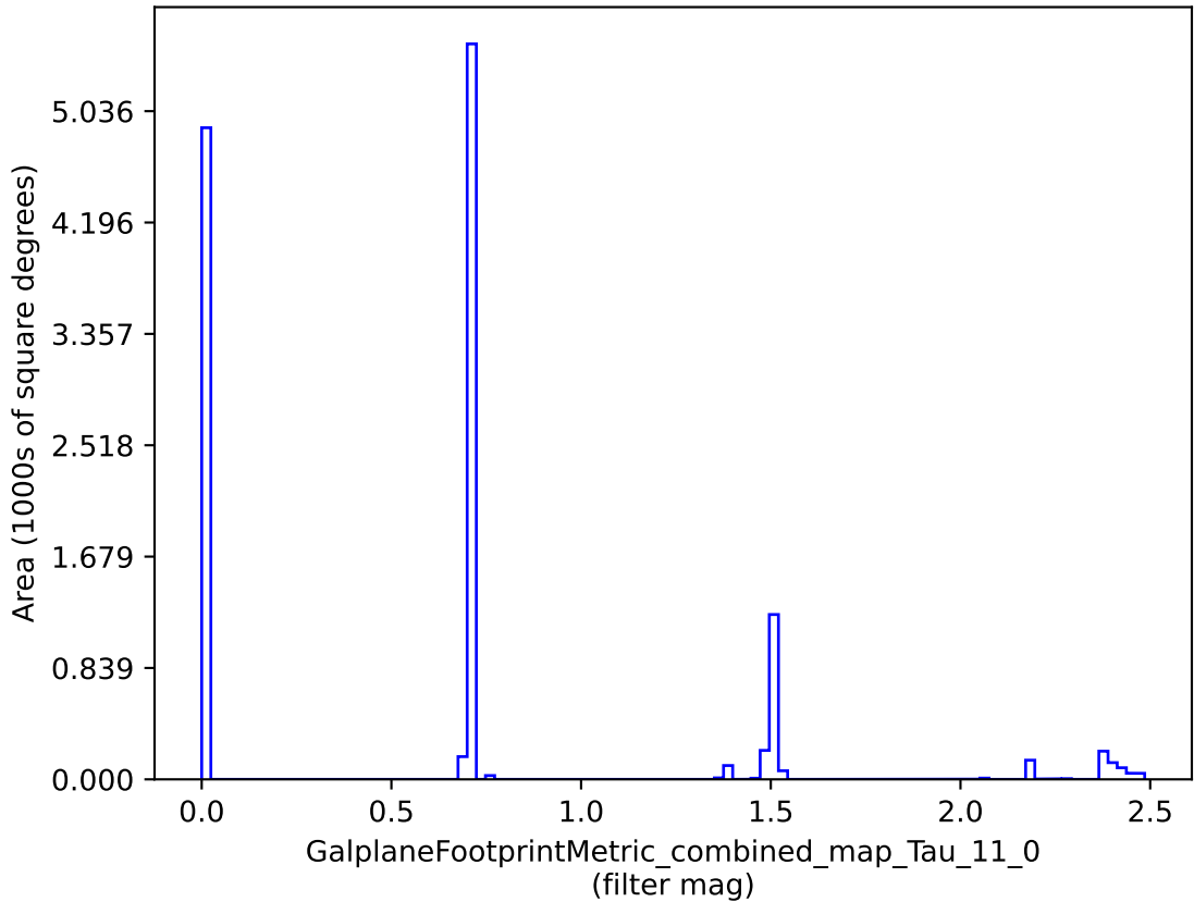
weather_cloudso30v3.4_10yrs : GalplaneFootprintMetric_combined_map_Tau_11_0
