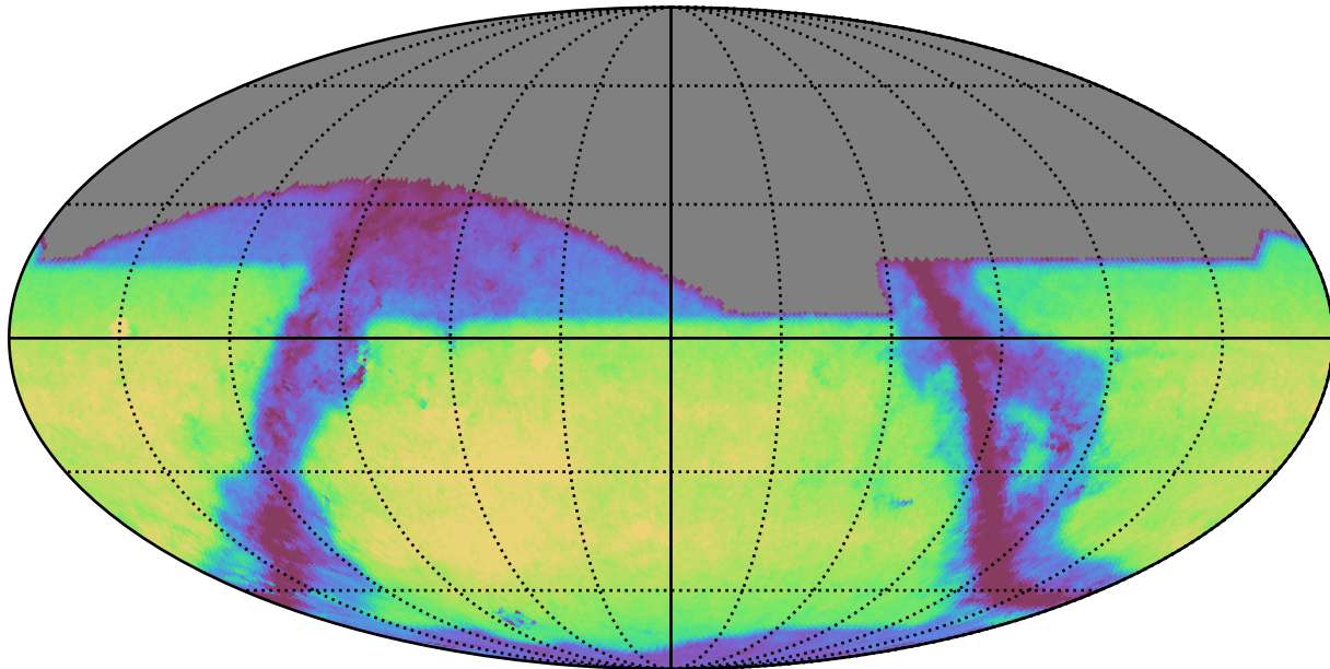
weather_cloudso30v3.4_10yrs z: GalaxyCountsMetricExtended
