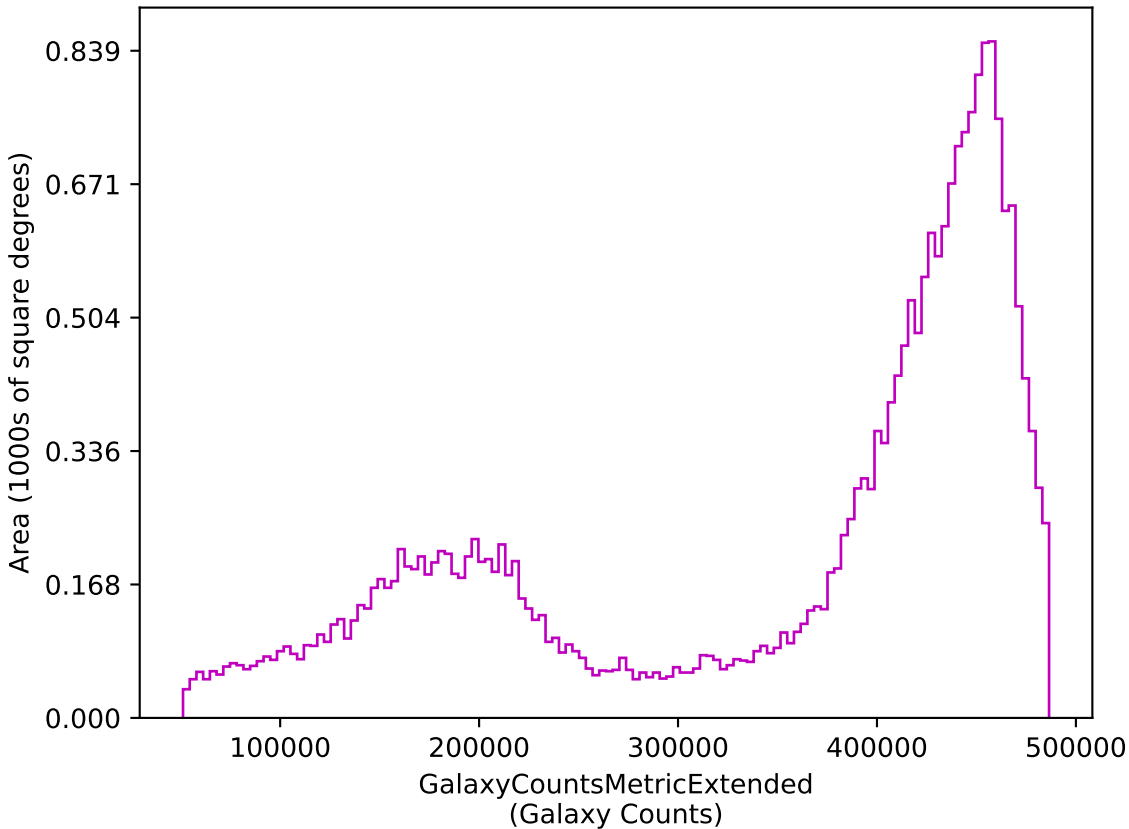
weather_cloudso30v3.4_10yrs z: GalaxyCountsMetricExtended
