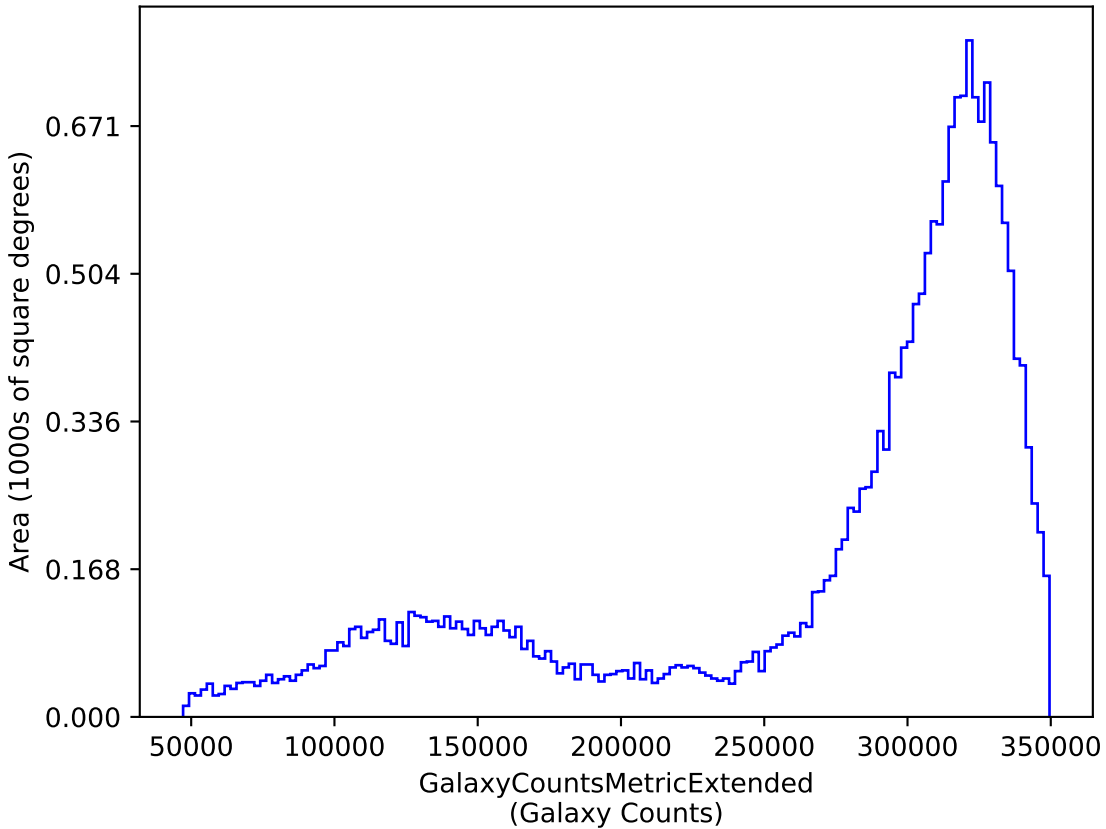
weather_cloudso30v3.4_10yrs y: GalaxyCountsMetricExtended
