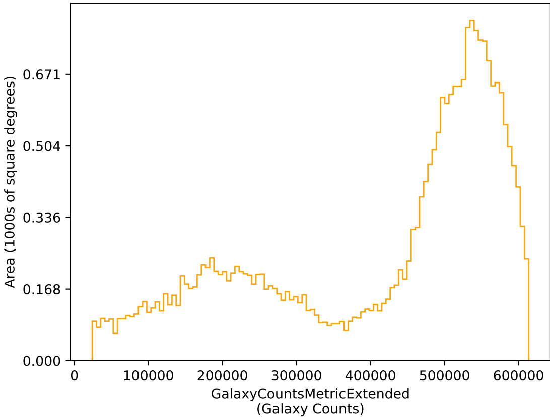
weather_cloudso30v3.4_10yrs r: GalaxyCountsMetricExtended
