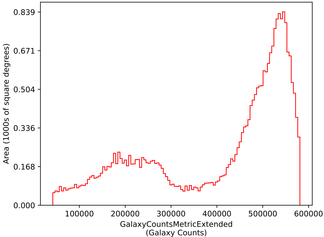
weather_cloudso30v3.4_10yrs i: GalaxyCountsMetricExtended
