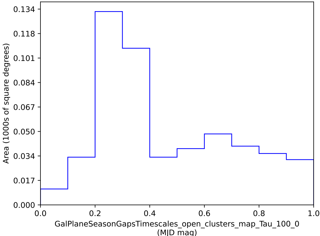
weather_cloudso30v3.4_10yrs : GalPlaneSeasonGapsTimescales_open_clusters_map_Tau_100_0
