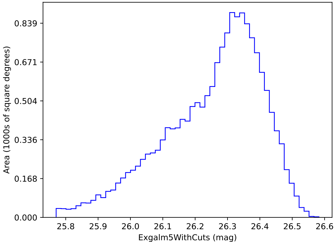
weather_cloudso30v3.4_10yrs i band non-DD year 8: ExgalM5WithCuts
