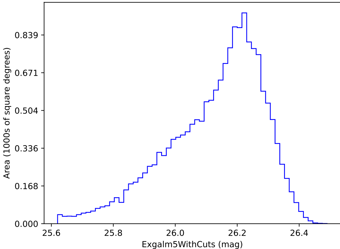
weather_cloudso30v3.4_10yrs i band non-DD year 6: ExgalM5WithCuts
