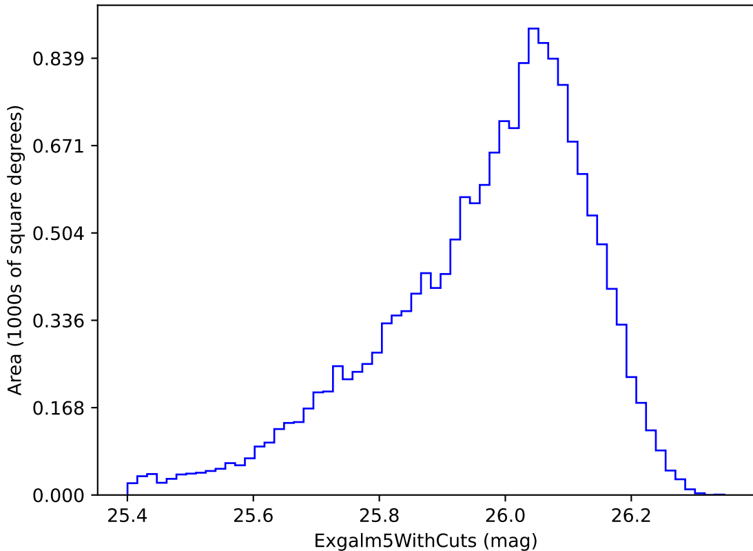
weather_cloudso30v3.4_10yrs i band non-DD year 4: ExgalM5WithCuts
