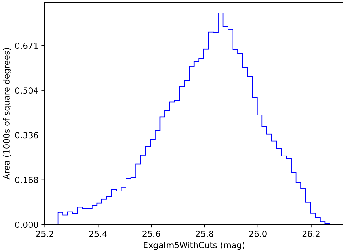
weather_cloudso30v3.4_10yrs i band non-DD year 3: ExgalM5WithCuts
