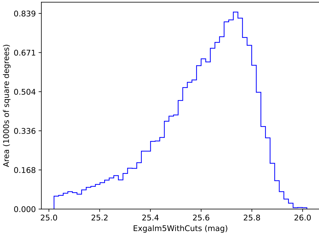
weather_cloudso30v3.4_10yrs i band non-DD year 2: ExgalM5WithCuts
