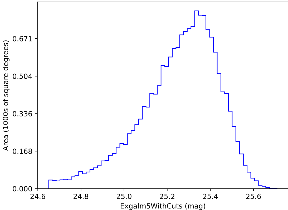
weather_cloudso30v3.4_10yrs i band non-DD year 1: ExgalM5WithCuts
