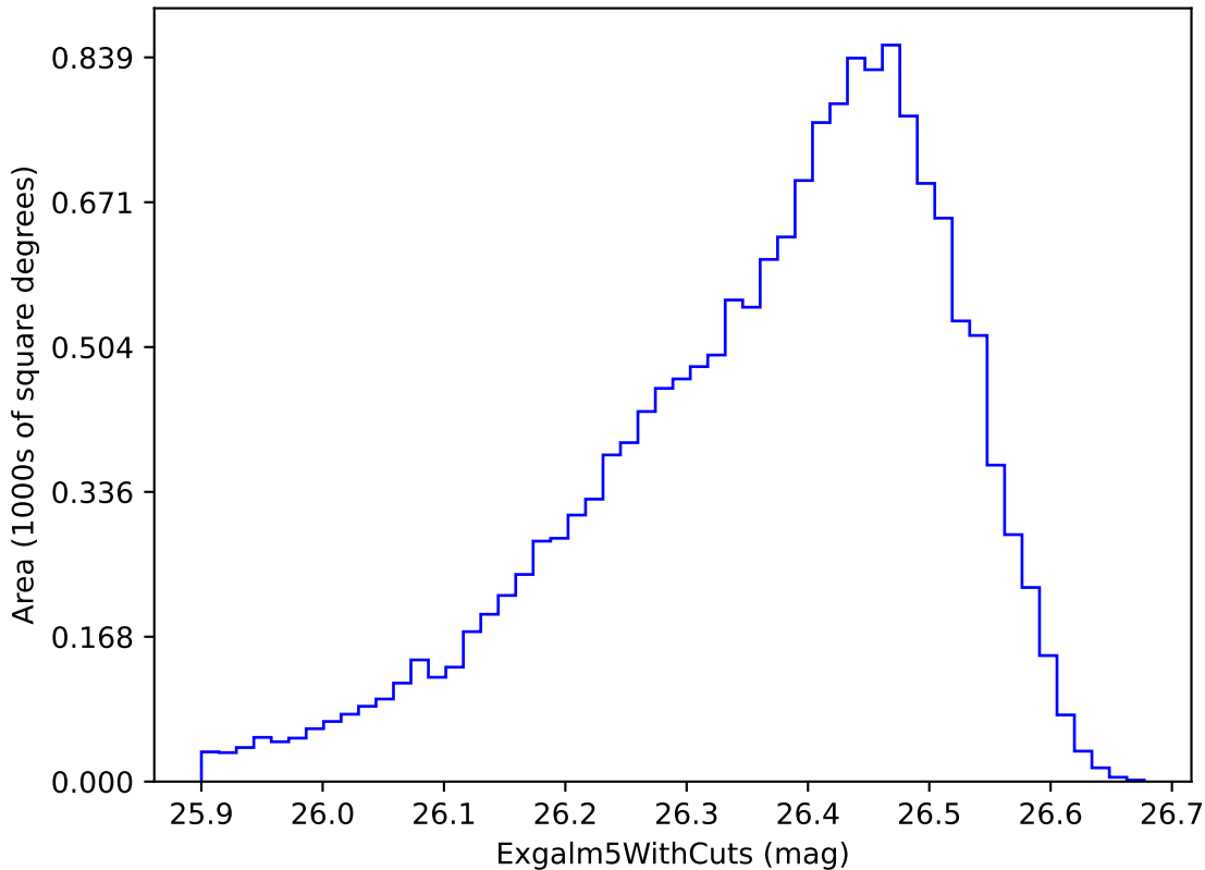
weather_cloudso30v3.4_10yrs i band non-DD year 10: Exgalml5WithCuts
