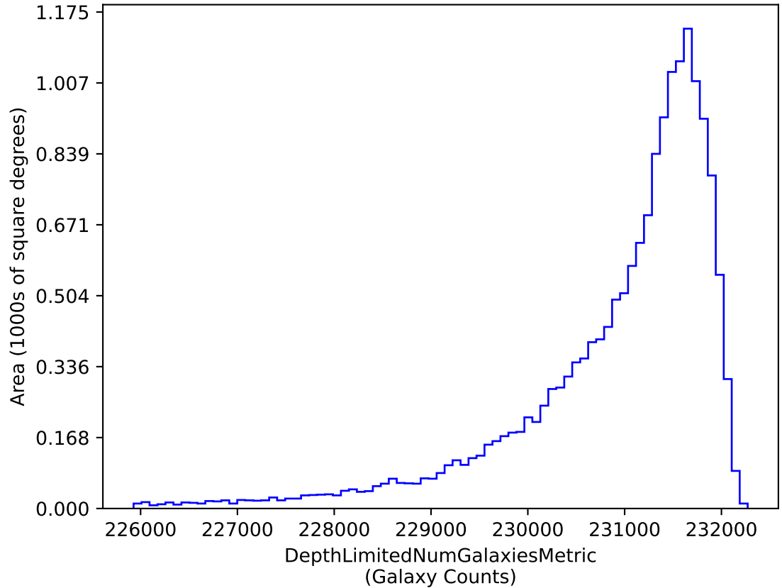
weather_cloudso30v3.4_10yrs i band galaxies non-DD: DepthLimitedNumGalaxiesMetric
