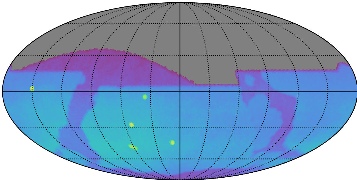
weather_cloudso30v3.4_10yrs : Brown Dwarf, L7
