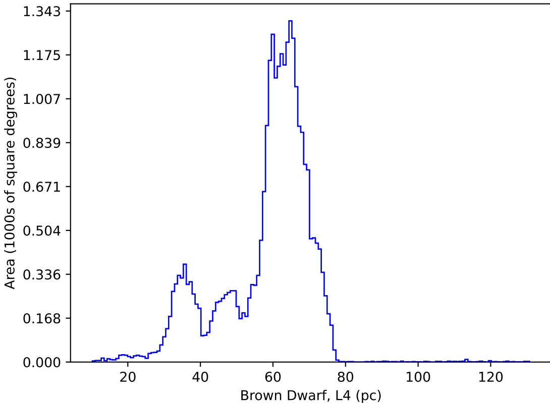
weather_cloudso30v3.4_10yrs : Brown Dwarf, L4
