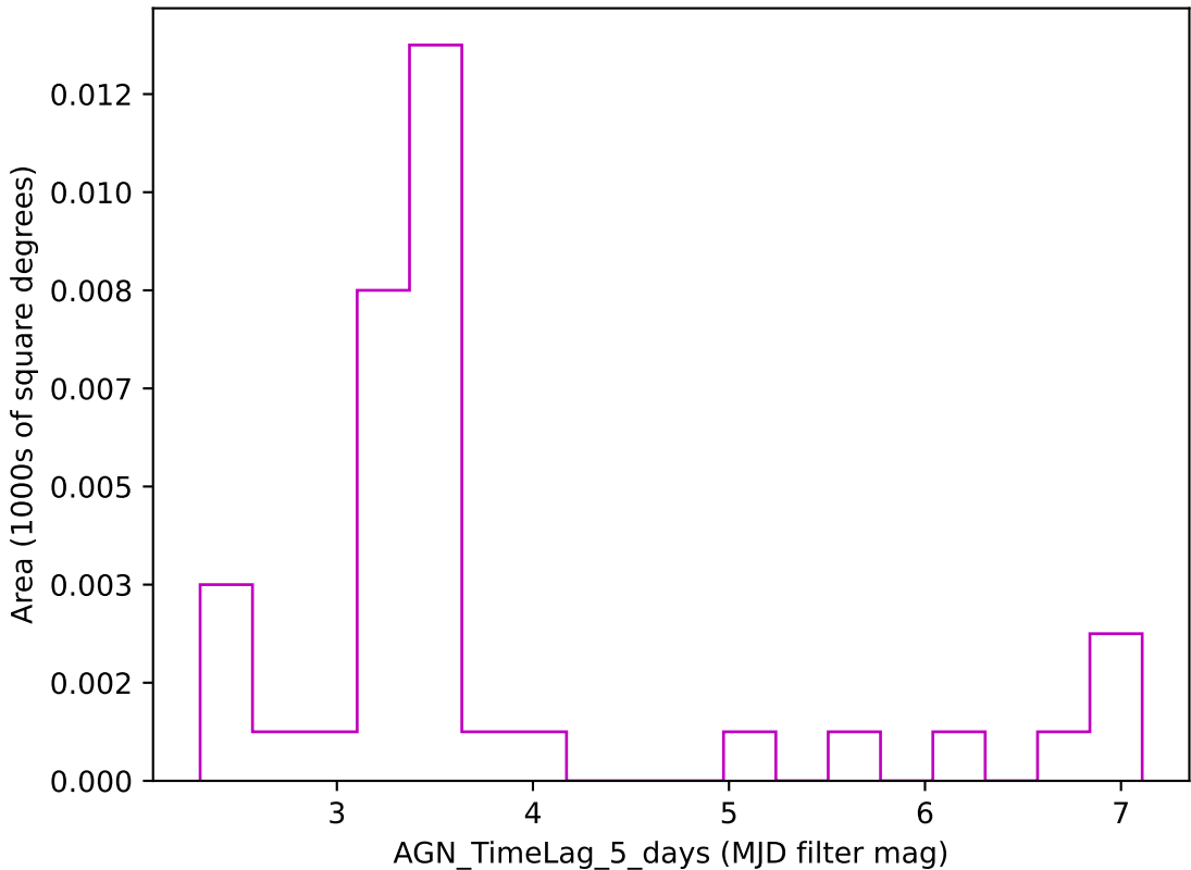
weather_cloudso30v3.4_10yrs z band: AGN_TimeLag_5_days
