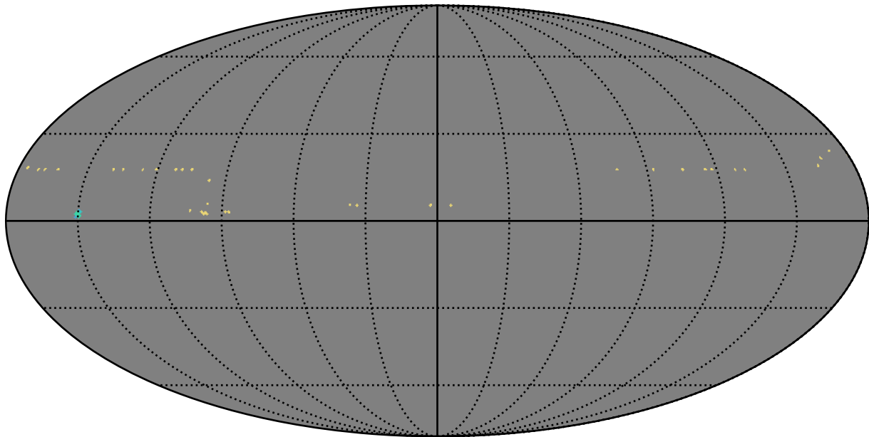
weather_cloudso30v3.4_10yrs y band: AGN_TimeLag_5_days
