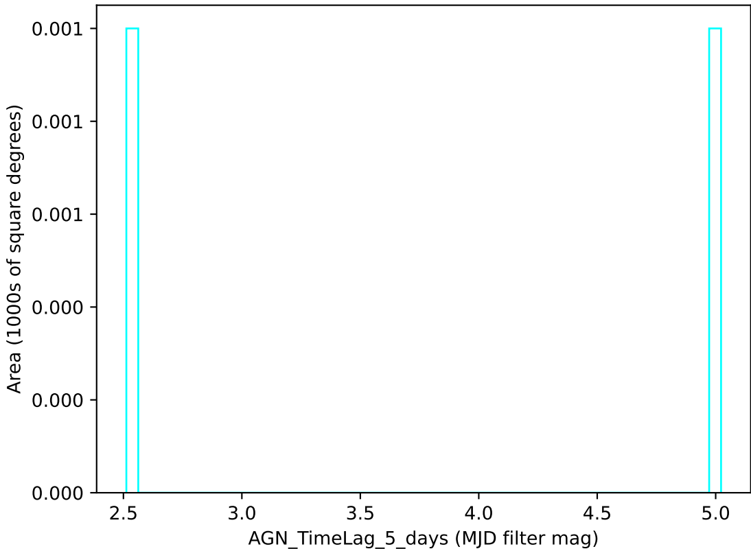
weather_cloudso30v3.4_10yrs u band: AGN_TimeLag_5_days
