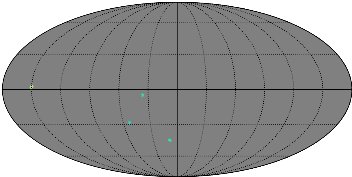
weather_cloudso30v3.4_10yrs r band: AGN_TimeLag_5_days
