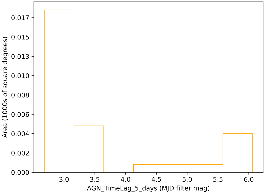
weather_cloudso30v3.4_10yrs r band: AGN_TimeLag_5_days
