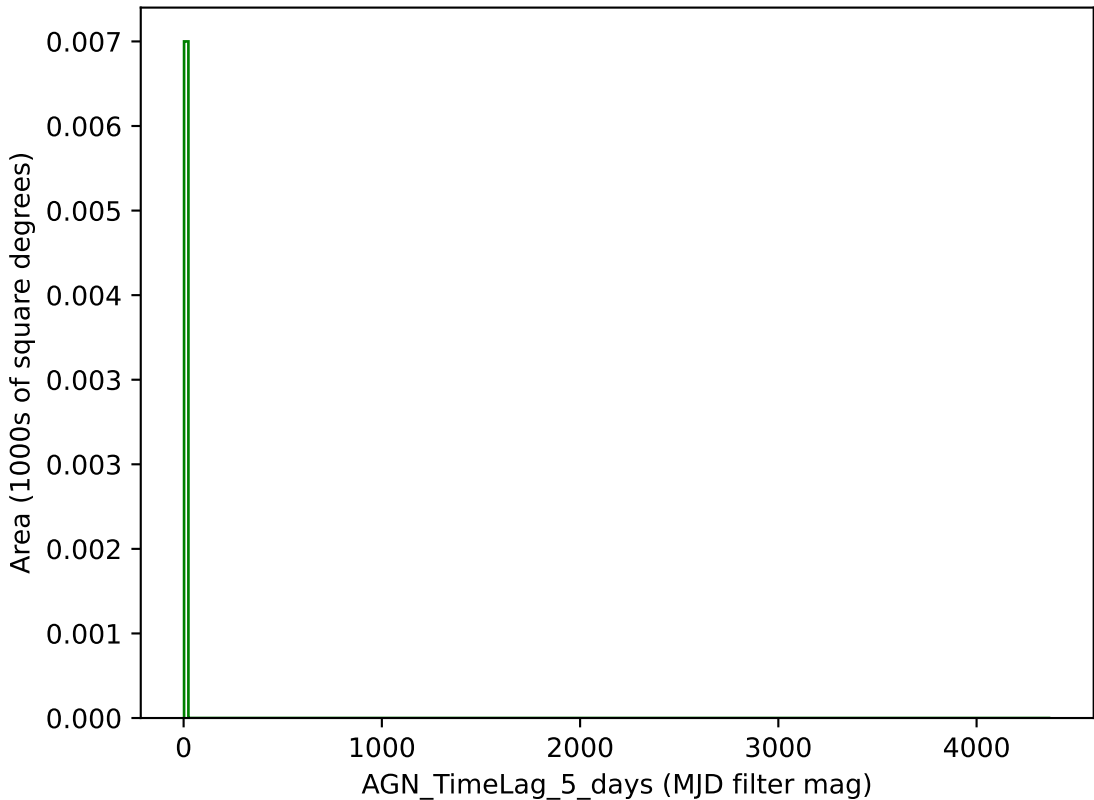
weather_cloudso30v3.4_10yrs g band: AGN_TimeLag_5_days
