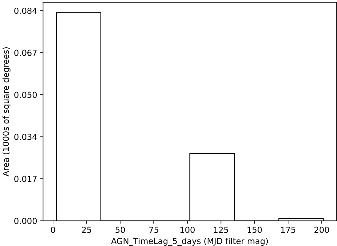
weather_cloudso30v3.4_10yrs all bands: AGN_TimeLag_5_days
