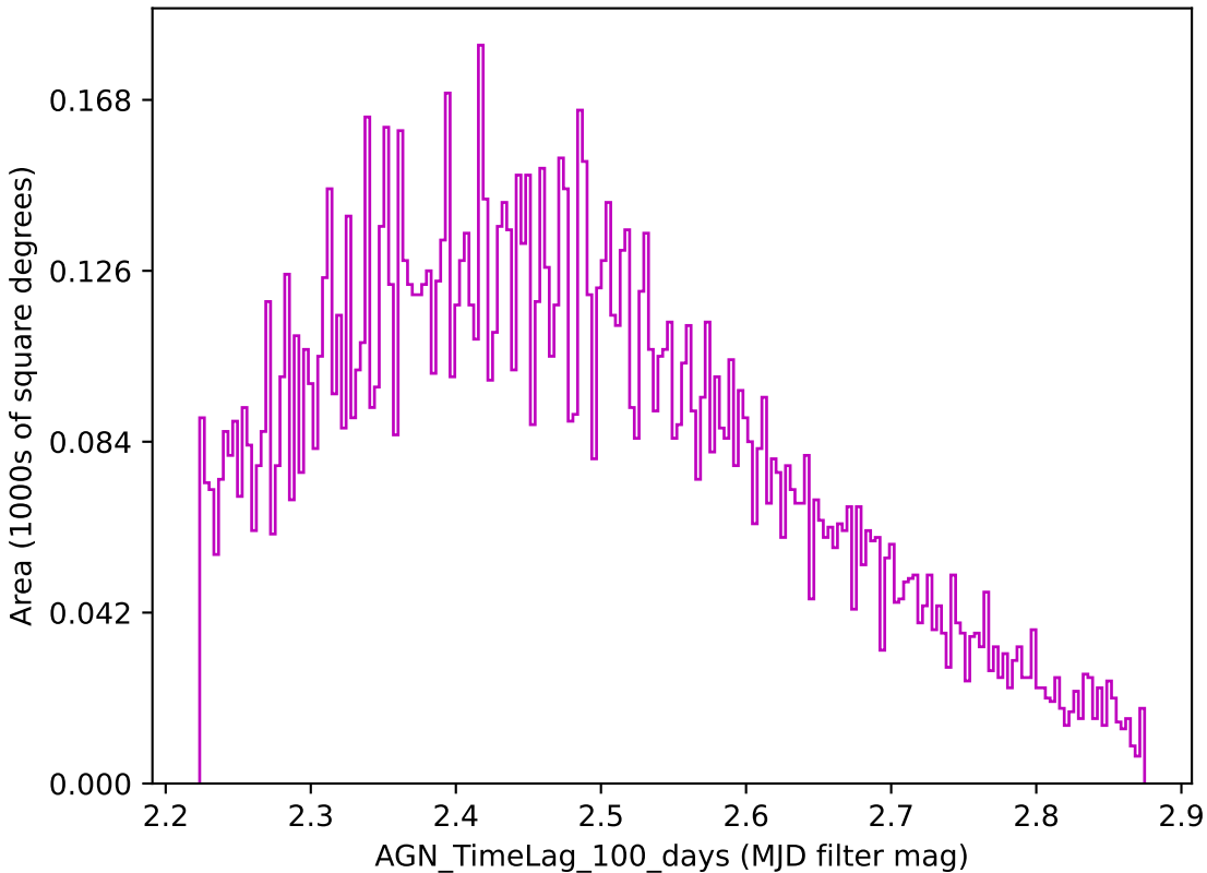
weather_cloudso30v3.4_10yrs z band: AGN_TimeLag_100_days
