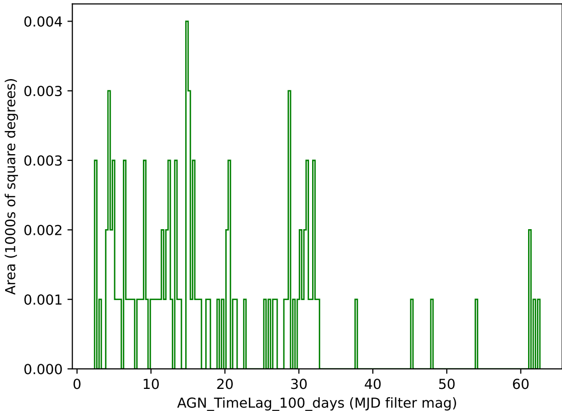
weather_cloudso30v3.4_10yrs g band: AGN_TimeLag_100_days
