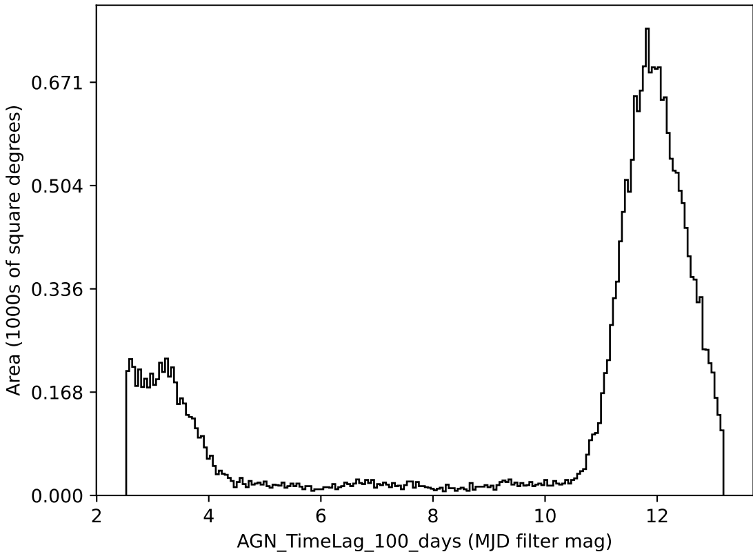
weather_cloudso30v3.4_10yrs all bands: AGN_TimeLag_100_days
