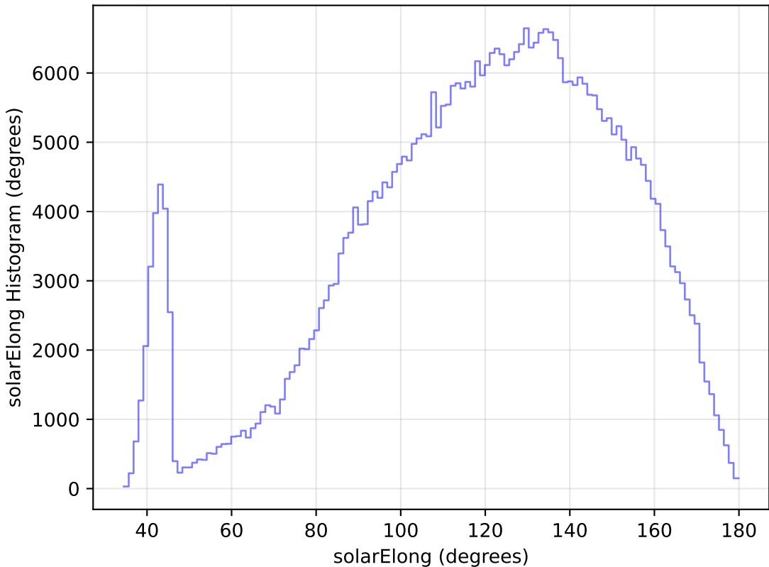
weather_cloudso30v3.4_10yrs WFD z band: solarElong Histogram
