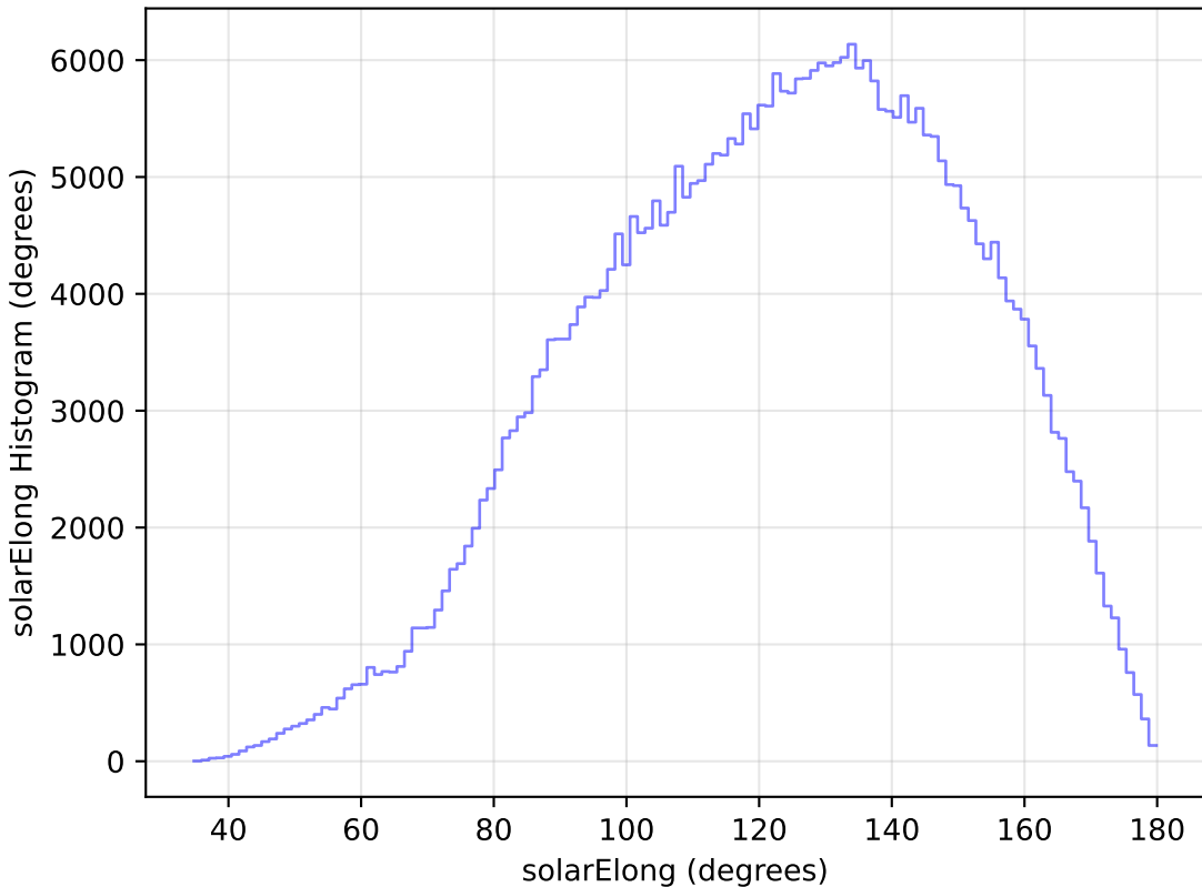
weather_cloudso30v3.4_10yrs WFD y band: solarElong Histogram
