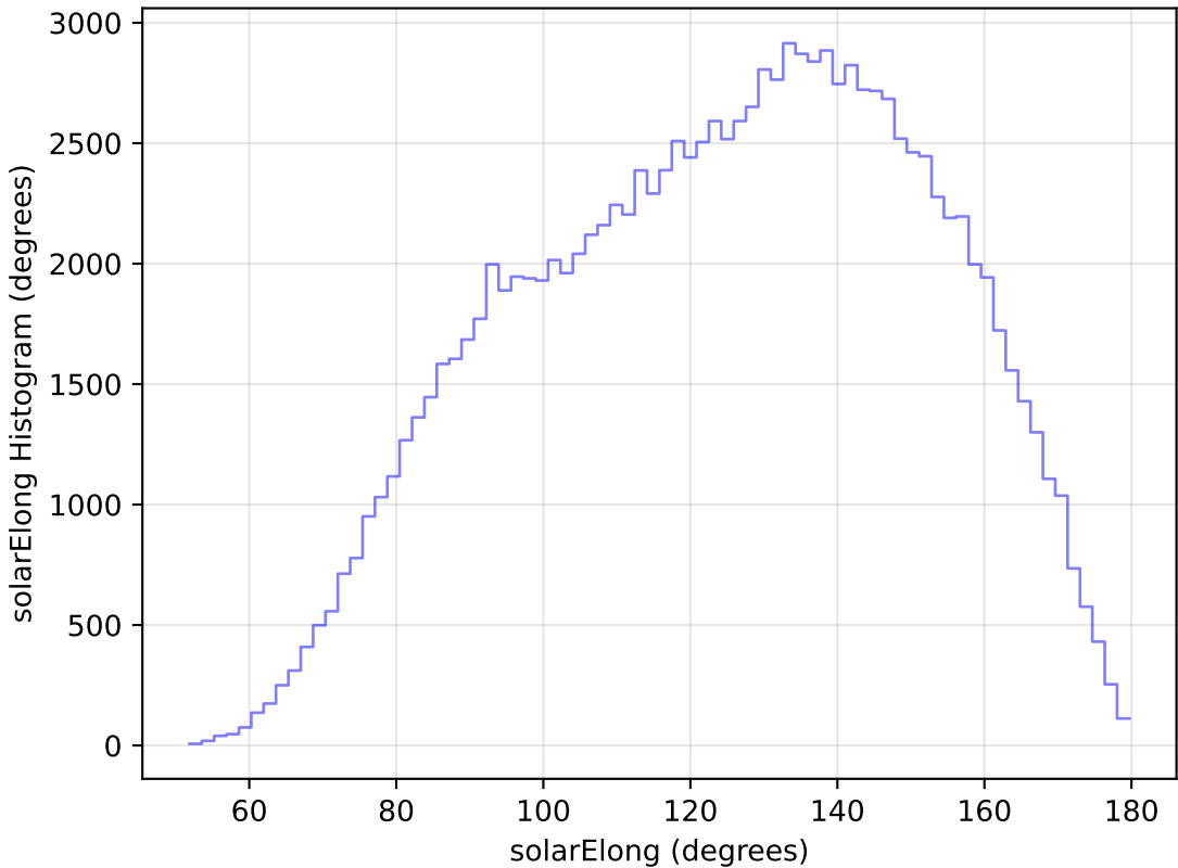
weather_cloudso30v3.4_10yrs WFD u band: solarElong Histogram
