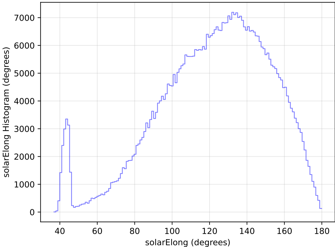
weather_cloudso30v3.4_10yrs WFD r band: solarElong Histogram
