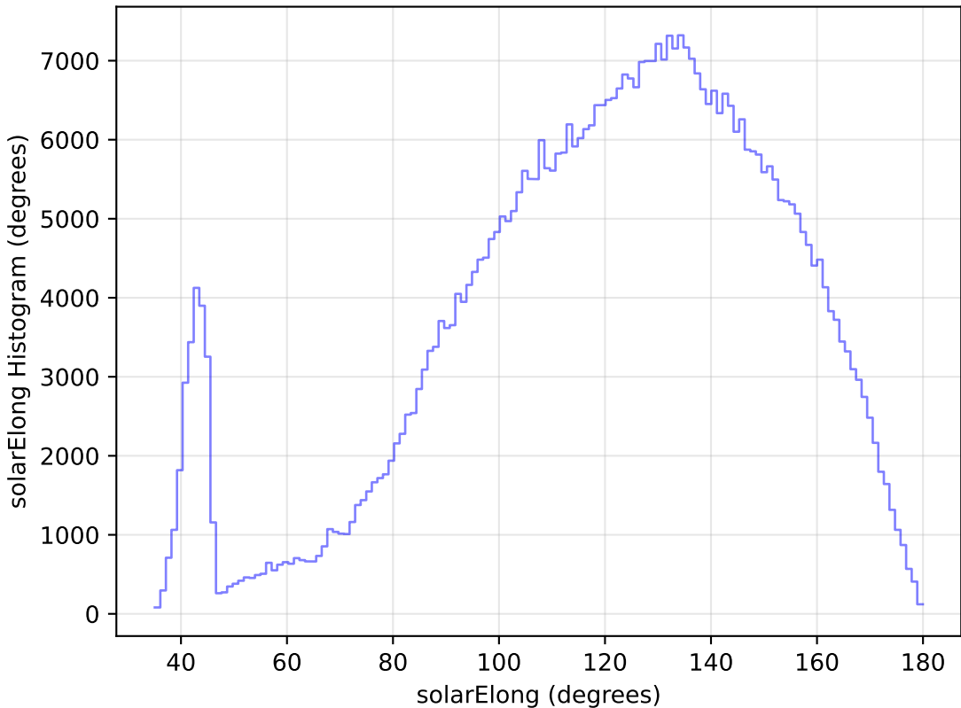
weather_cloudso30v3.4_10yrs WFD i band: solarElong Histogram
