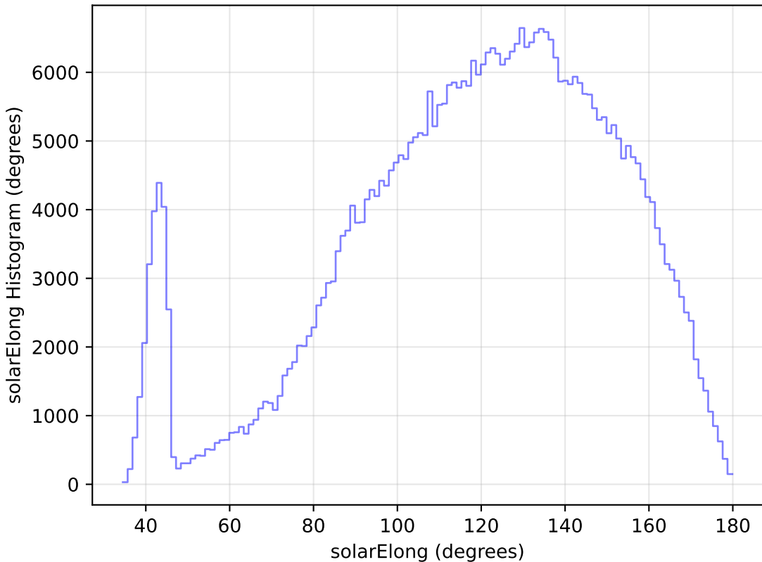
weather_cloudso30v3.4_10yrs All sky z band: solarElong Histogram
