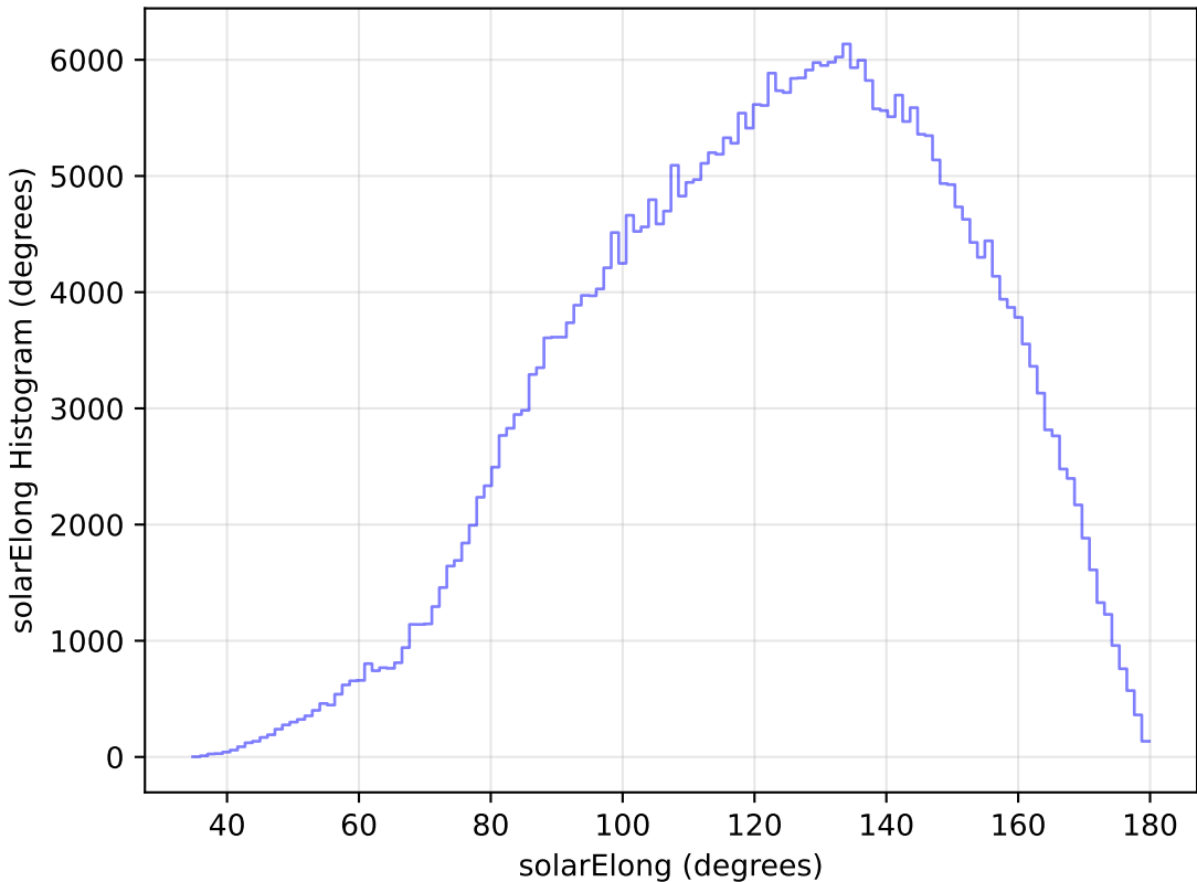
weather_cloudso30v3.4_10yrs All sky y band: solarElong Histogram
