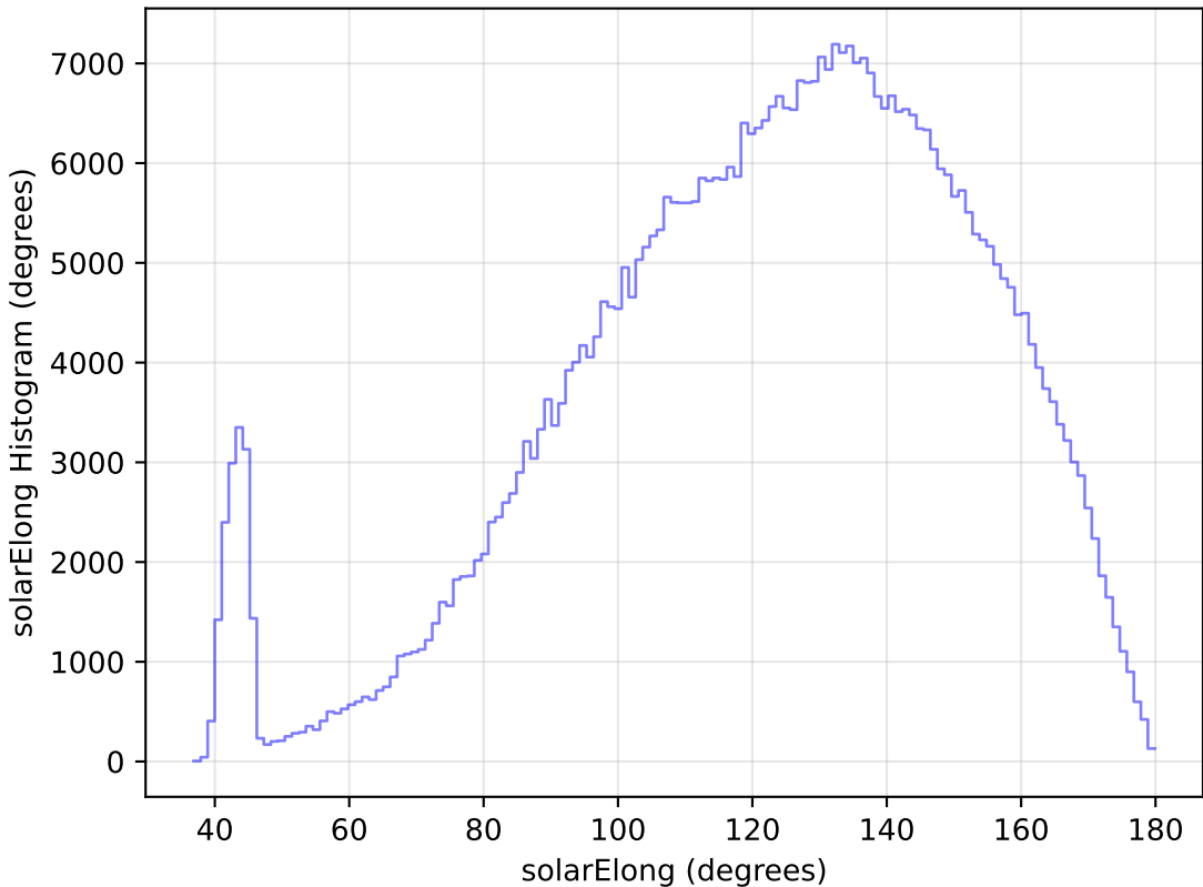
weather_cloudso30v3.4_10yrs All sky r band: solarElong Histogram
