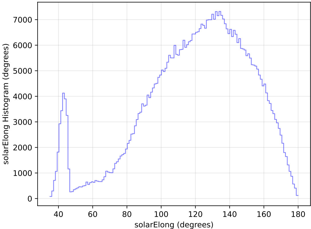
weather_cloudso30v3.4_10yrs All sky i band: solarElong Histogram
