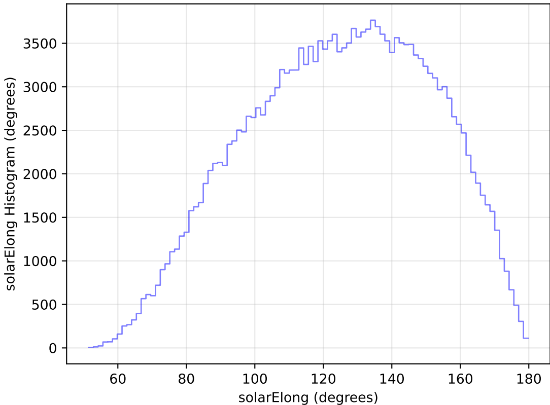
weather_cloudso30v3.4_10yrs All sky g band: solarElong Histogram
