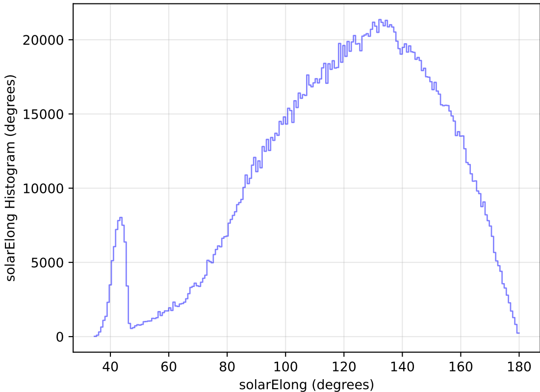
weather_cloudso30v3.4_10yrs All sky all bands: solarElong Histogram
