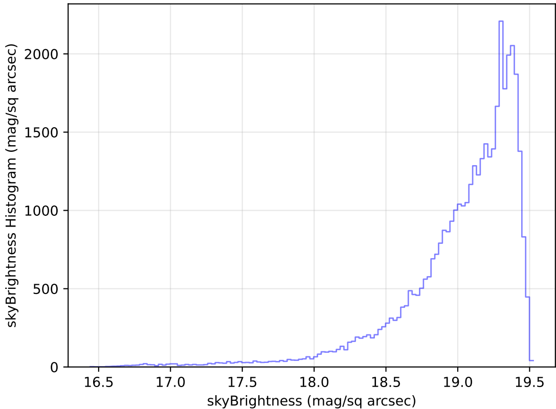
weather_cloudso30v3.4_10yrs Yr 1 z band: skyBrightness Histogram
