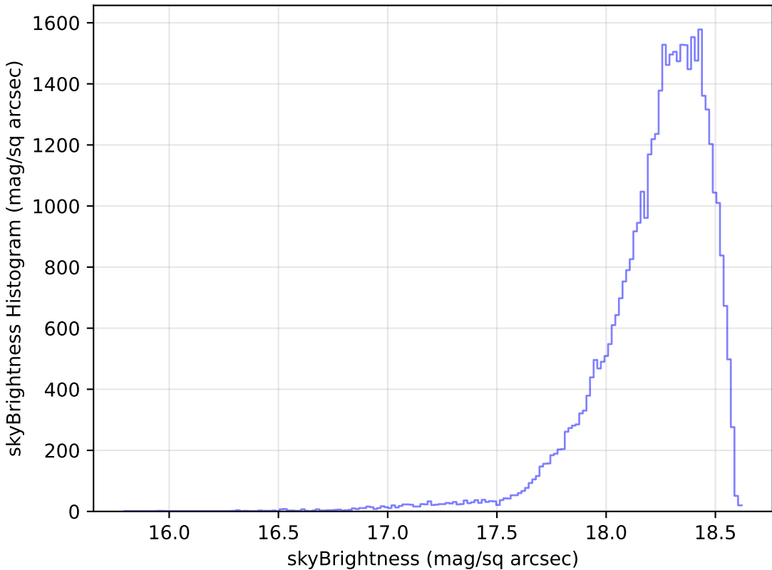
weather_cloudso30v3.4_10yrs Yr 1 y band: skyBrightness Histogram
