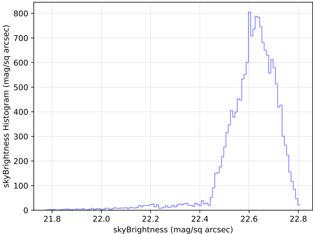
weather_cloudso30v3.4_10yrs Yr 1 u band: skyBrightness Histogram
