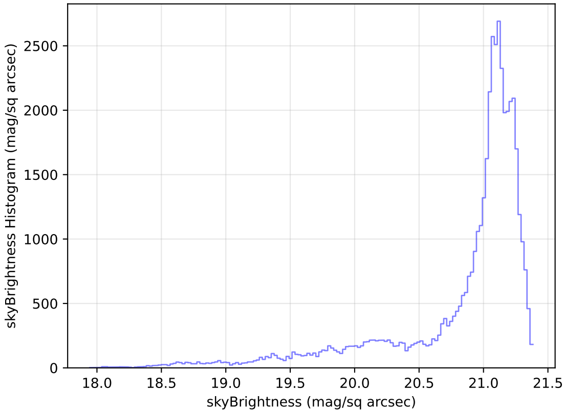
weather_cloudso30v3.4_10yrs Yr 1 r band: skyBrightness Histogram
