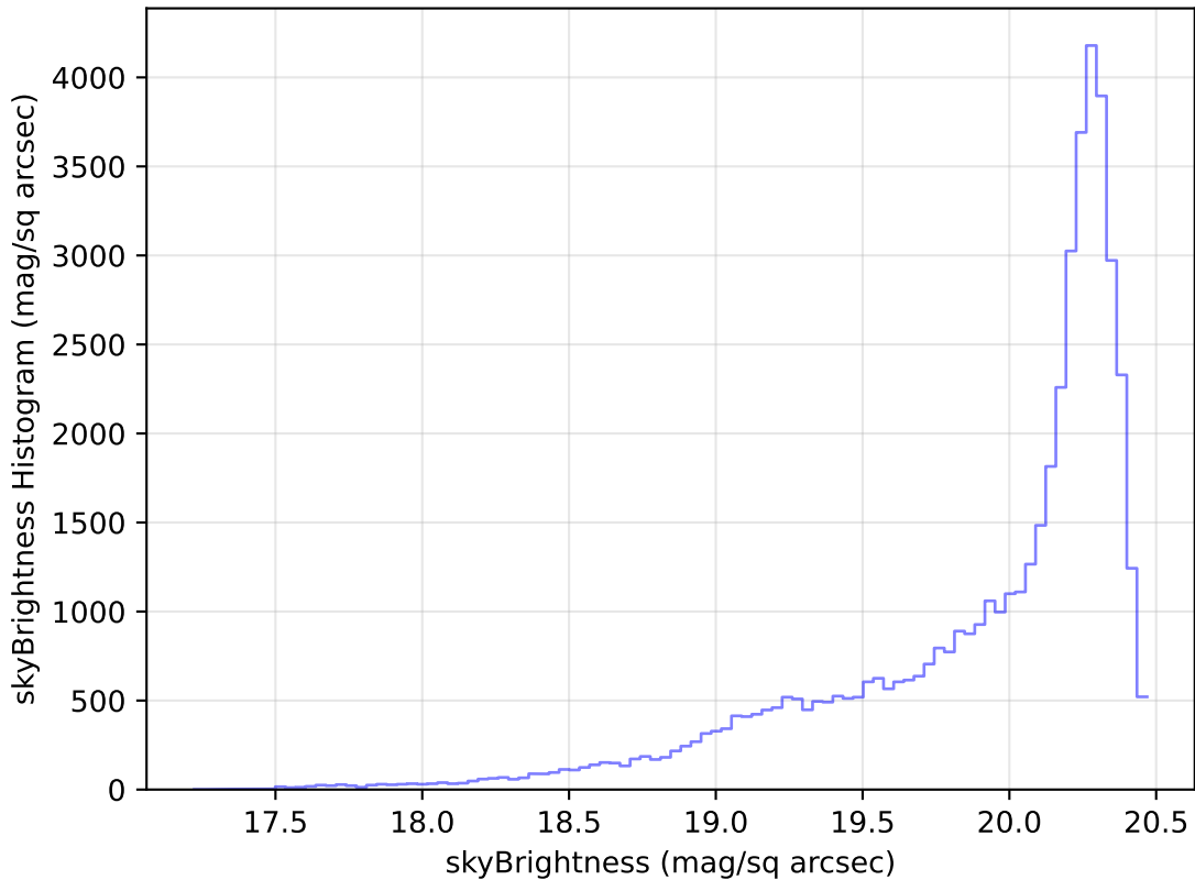
weather_cloudso30v3.4_10yrs Yr 1 i band: skyBrightness Histogram
