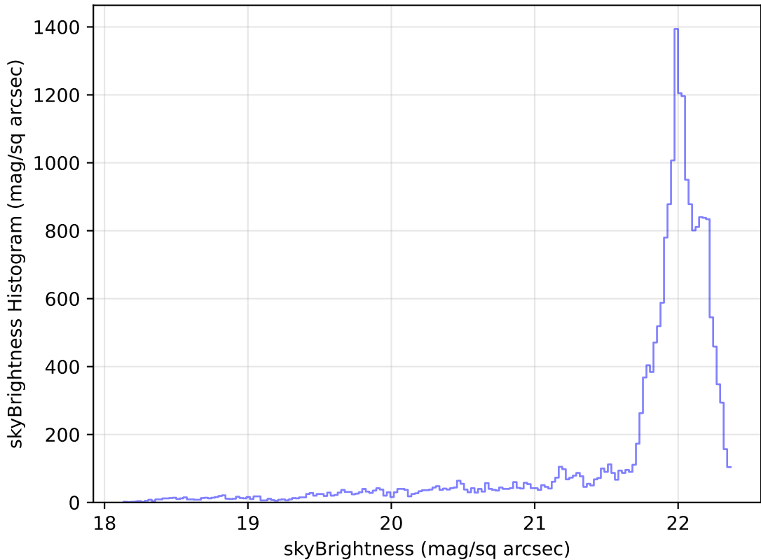
weather_cloudso30v3.4_10yrs Yr 1 g band: skyBrightness Histogram
