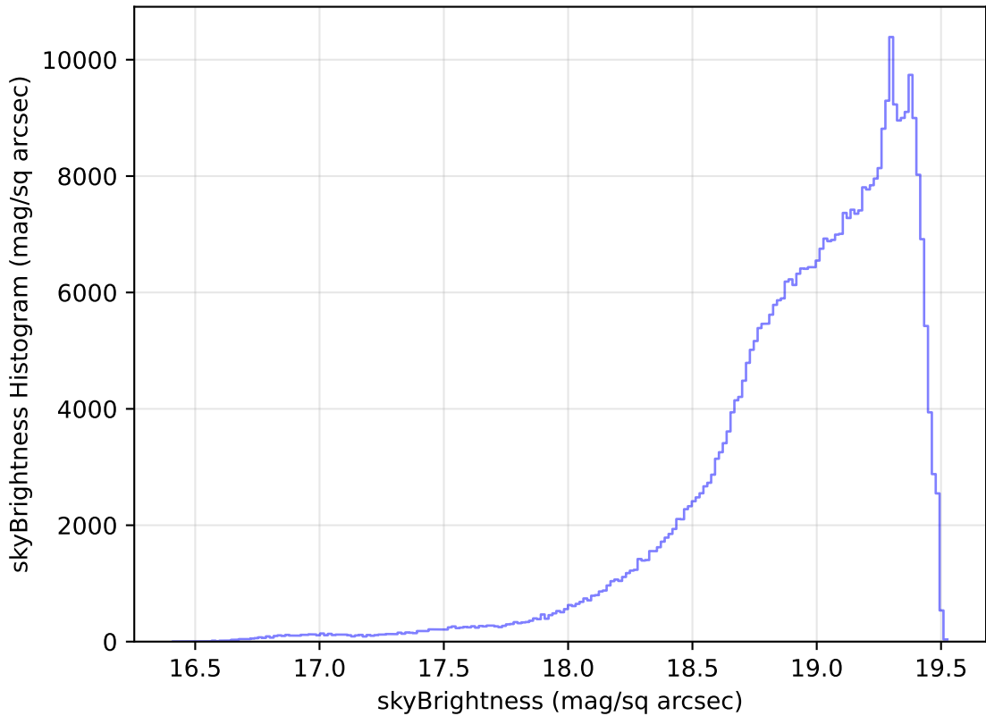
weather_cloudso30v3.4_10yrs WFD z band: skyBrightness Histogram
