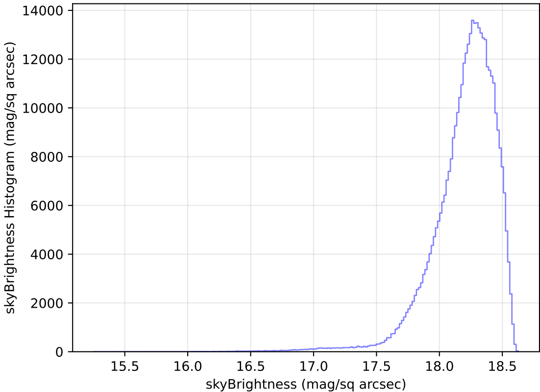
weather_cloudso30v3.4_10yrs WFD y band: skyBrightness Histogram
