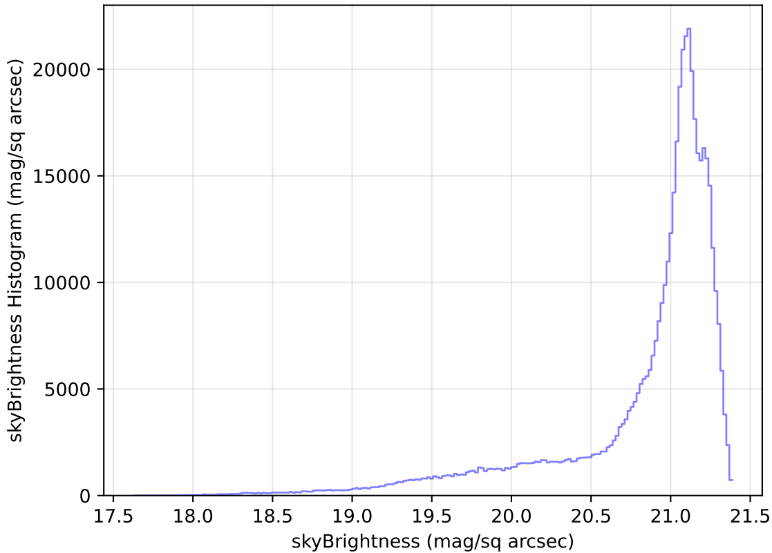
weather_cloudso30v3.4_10yrs WFD r band: skyBrightness Histogram
