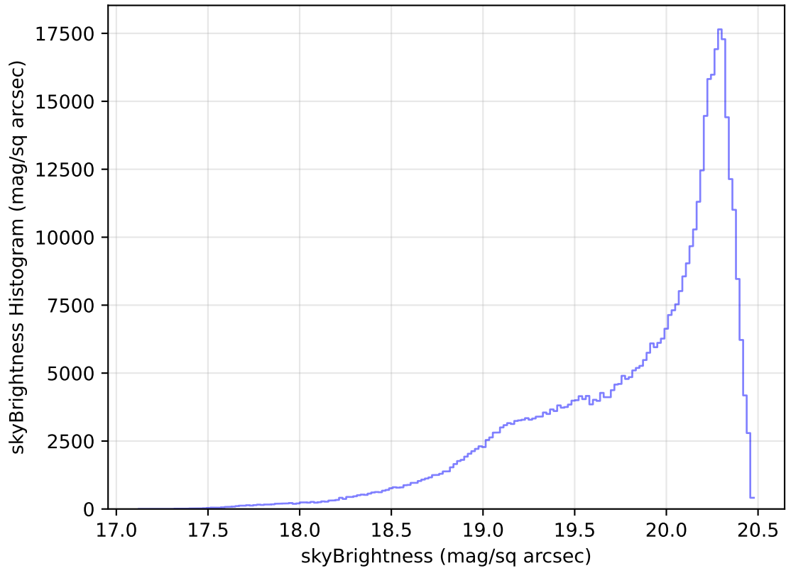
weather_cloudso30v3.4_10yrs WFD i band: skyBrightness Histogram
