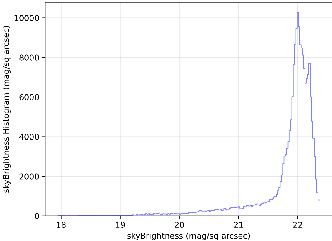
weather_cloudso30v3.4_10yrs WFD g band: skyBrightness Histogram
