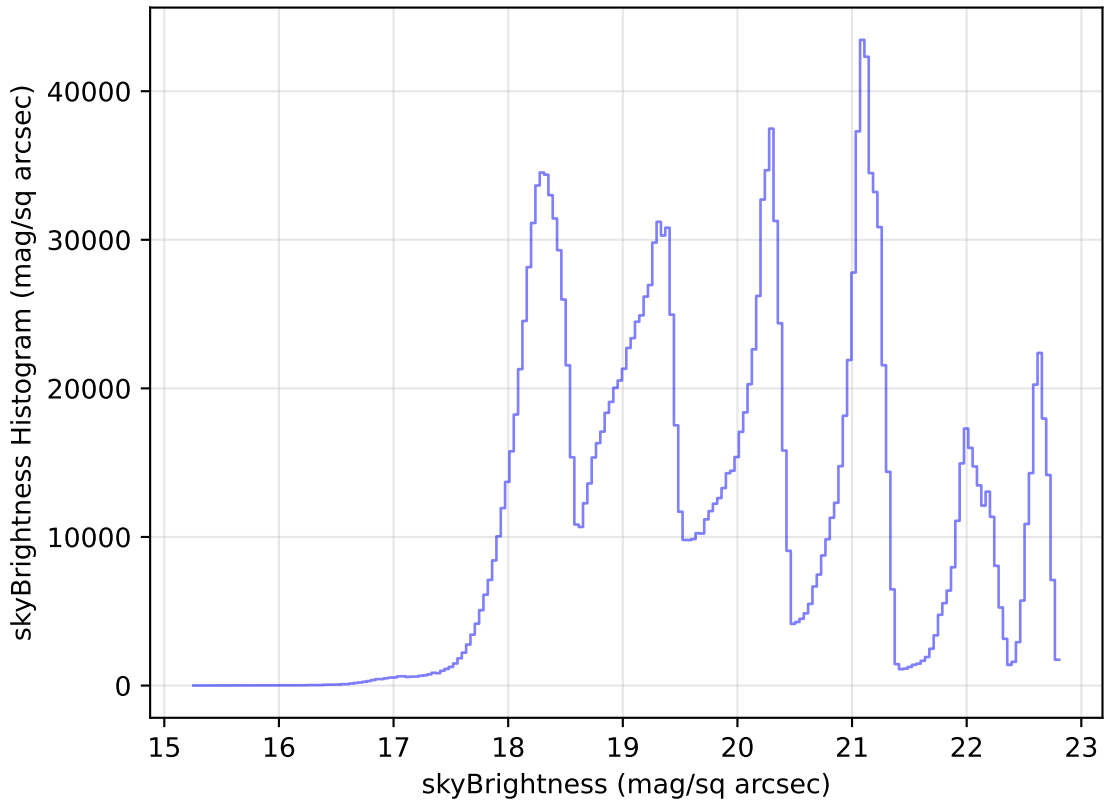
weather_cloudso30v3.4_10yrs WFD all bands: skyBrightness Histogram
